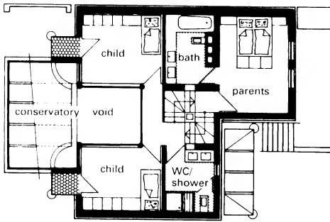
2 Upper floor
